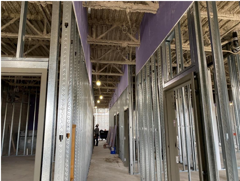
Installation of above ceiling drywall is continuing in the administrative offices as well as electrical rough-in work.
