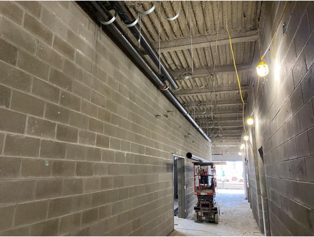
Installation of hydronic piping in the Locker Room corridor.
