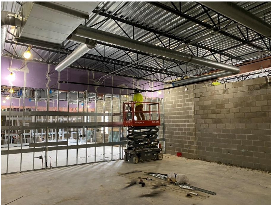
Above ceiling drywall joints are being finished in Area C.
