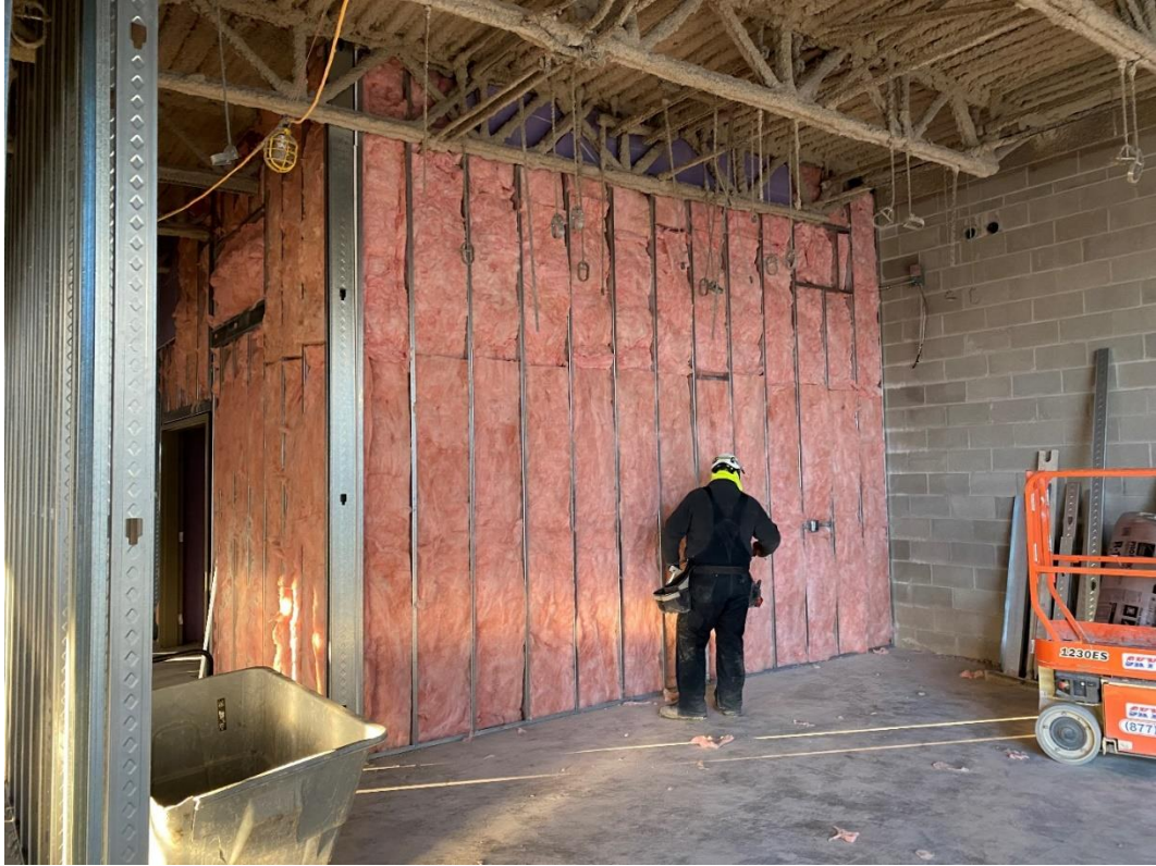
Installation of acoustical insulation in stud walls at Area A.
