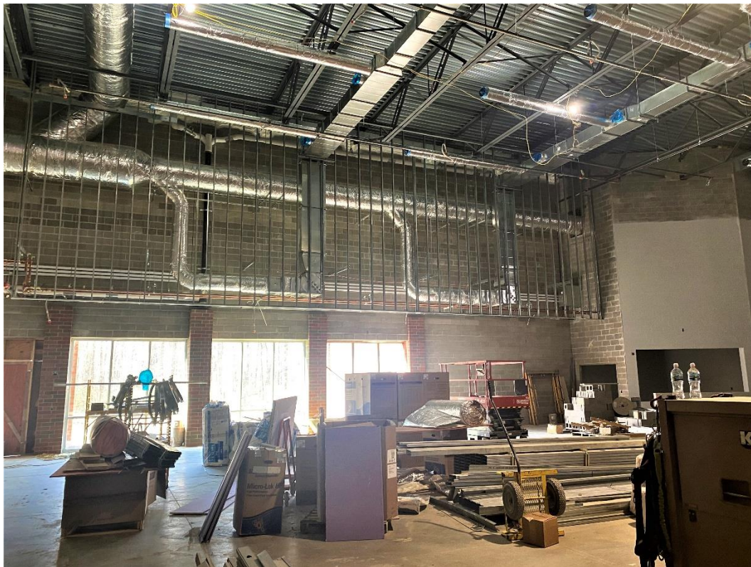
Light gauge metal framing for soffits is progressing in the Performing Arts Center.
