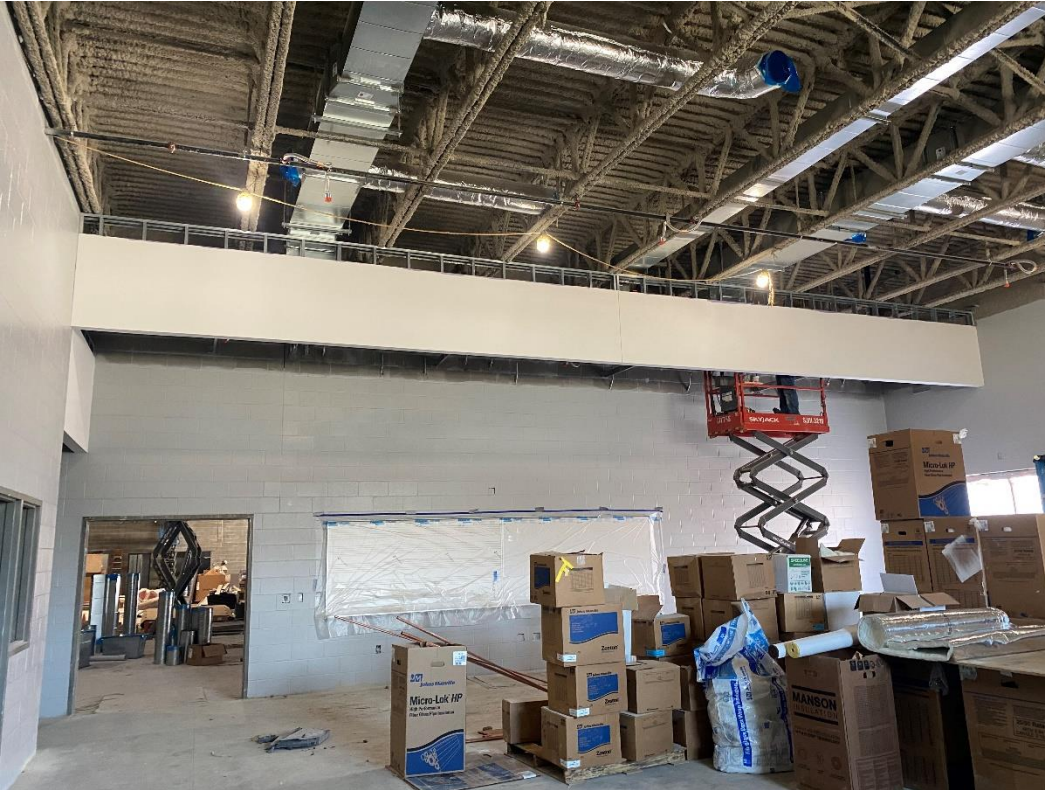
Drywall bulkhead is completed in the Instrumental Music Classroom.
