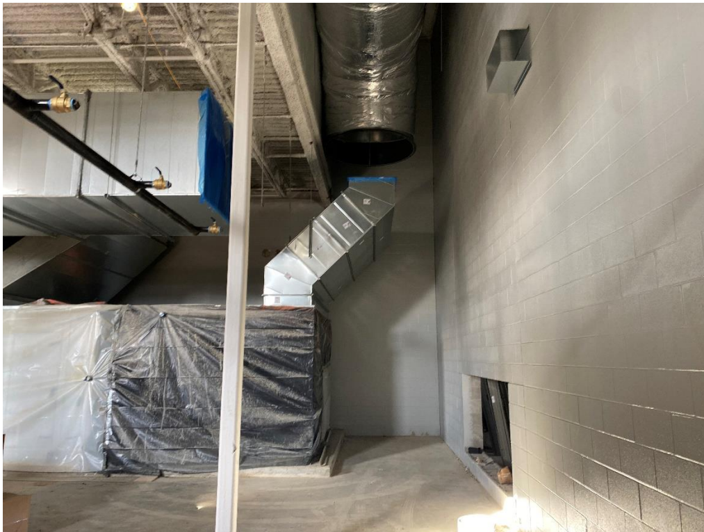
Main supply air ducts are ready for final connection to the air handler for the Gym.
