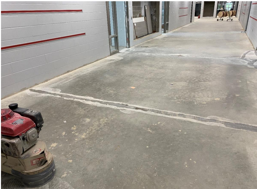
Control joints in the main corridor slab north of the main entry are ground and filled in preparation for epoxy flooring.
