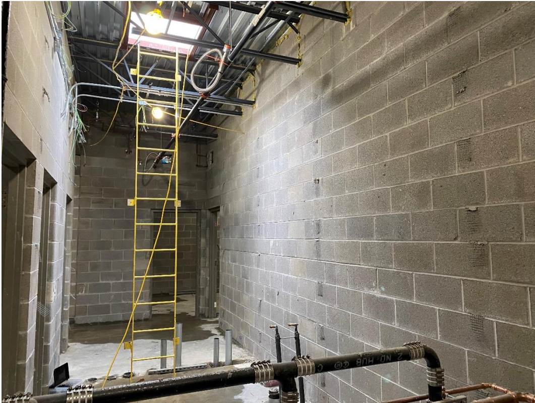
Masonry walls closed to the metal decking above in second-floor Area C toilet rooms.
