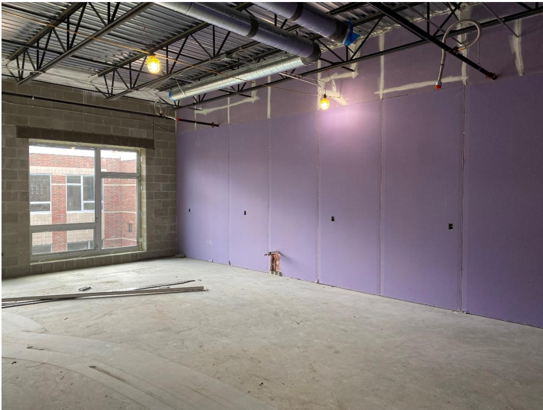
Installation of drywall continues to progress in second-floor Area D classrooms.
