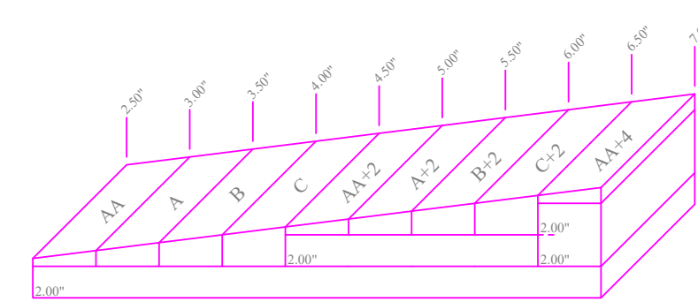
1/8" PER FOOT Tapered Detail
