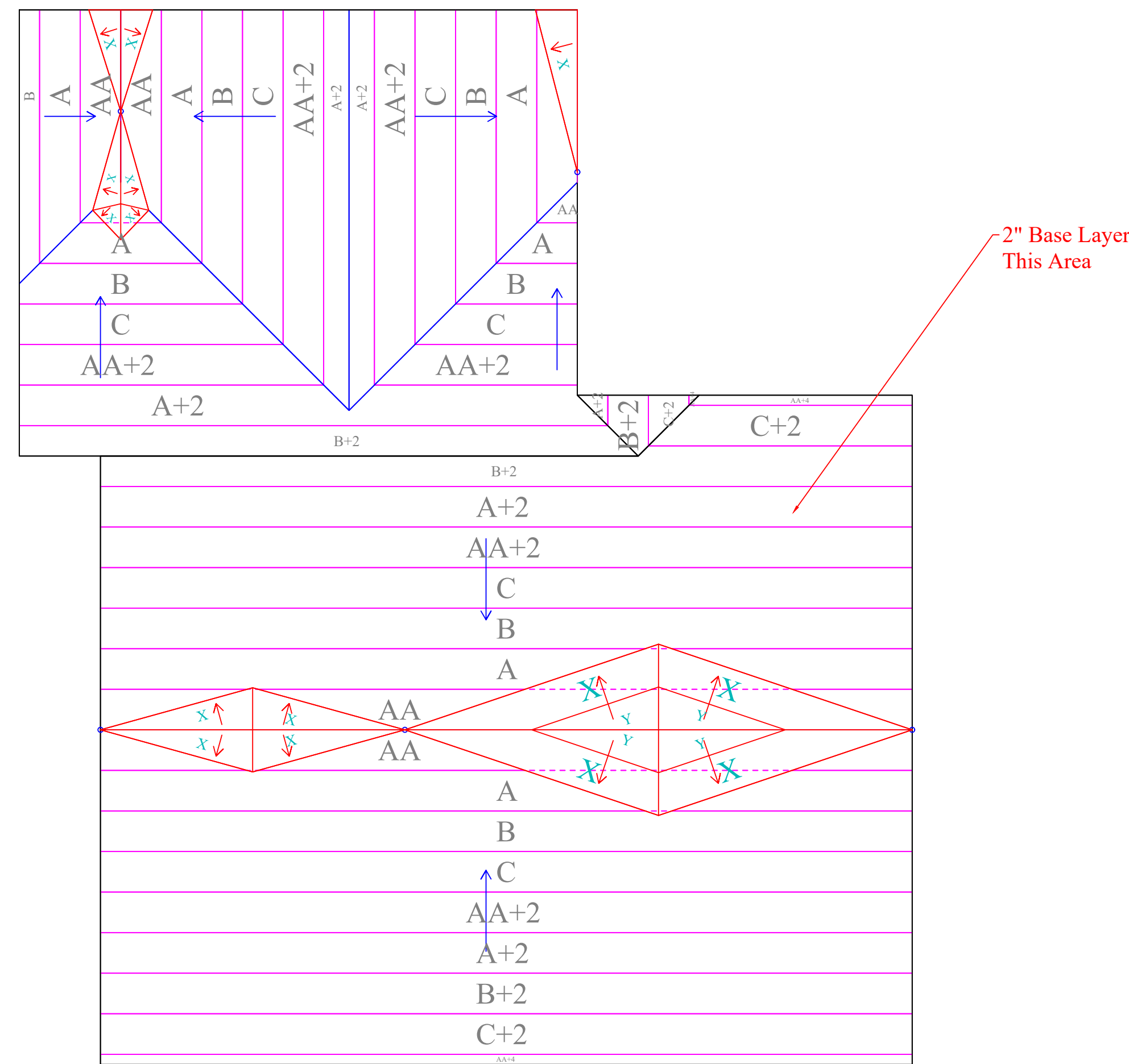
Area A Tapered Roof Plan
