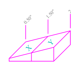
1/4" PER FOOT Cricket Detail
