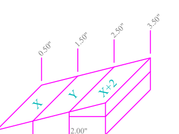
1/4" PER FOOT Cricket Detail
