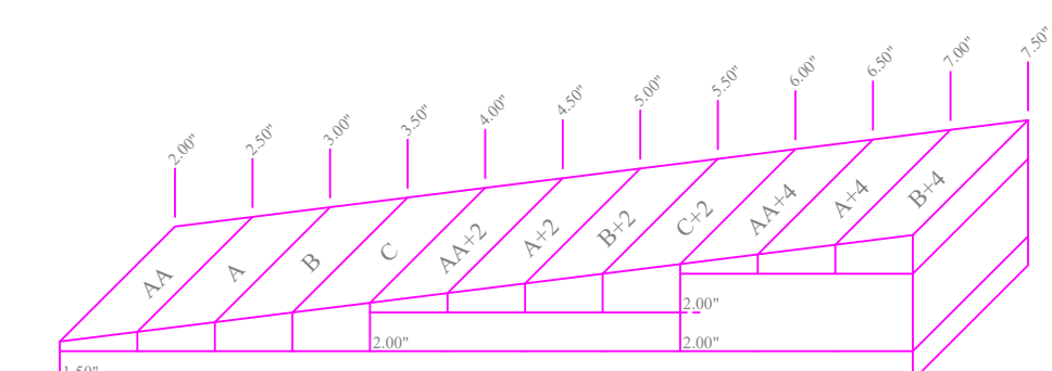
1/8" PER FOOT Tapered Detail
